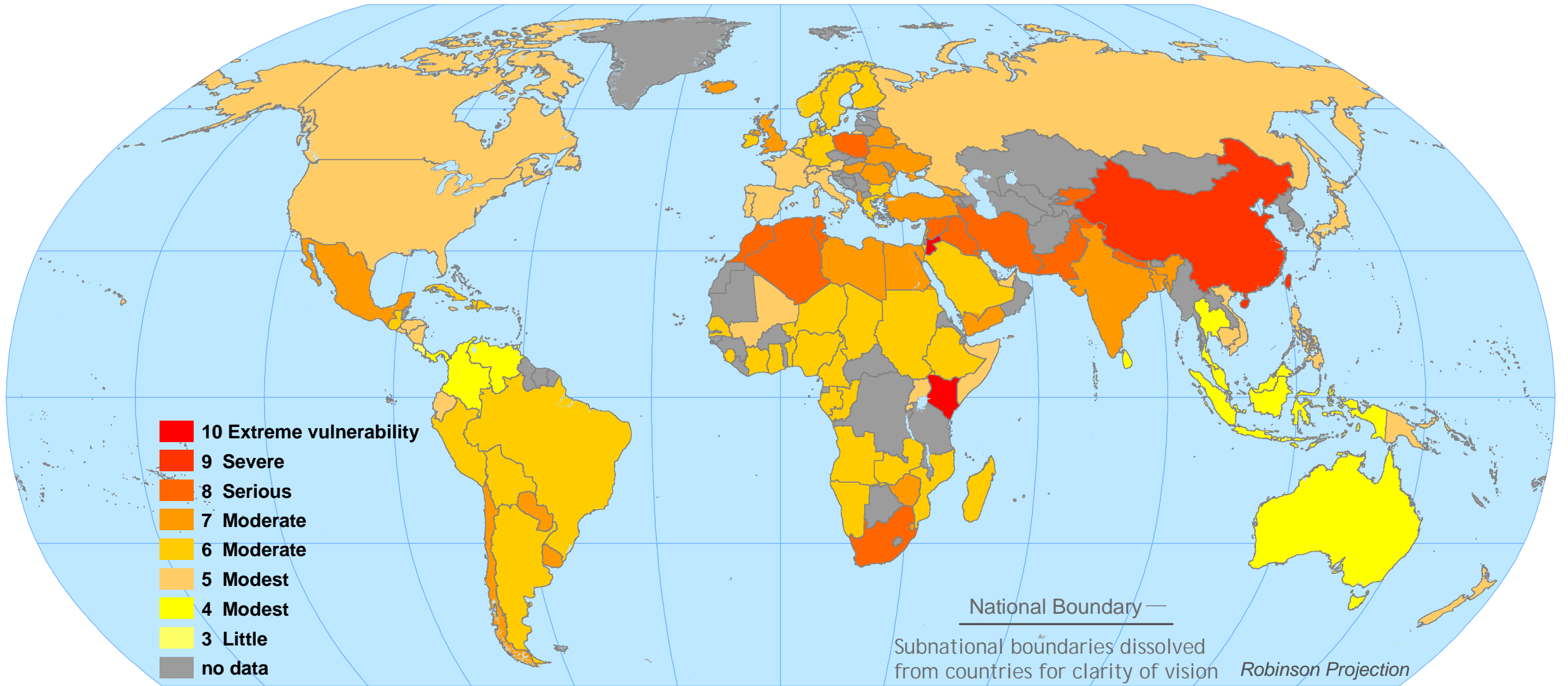
Scenario B2 in Year 2100 with Climate Sensitivity Equal to 5.5 Degrees C Annual Mean Temperature with Aggregate Impacts Calibration and Enhanced Adaptive Capacity
