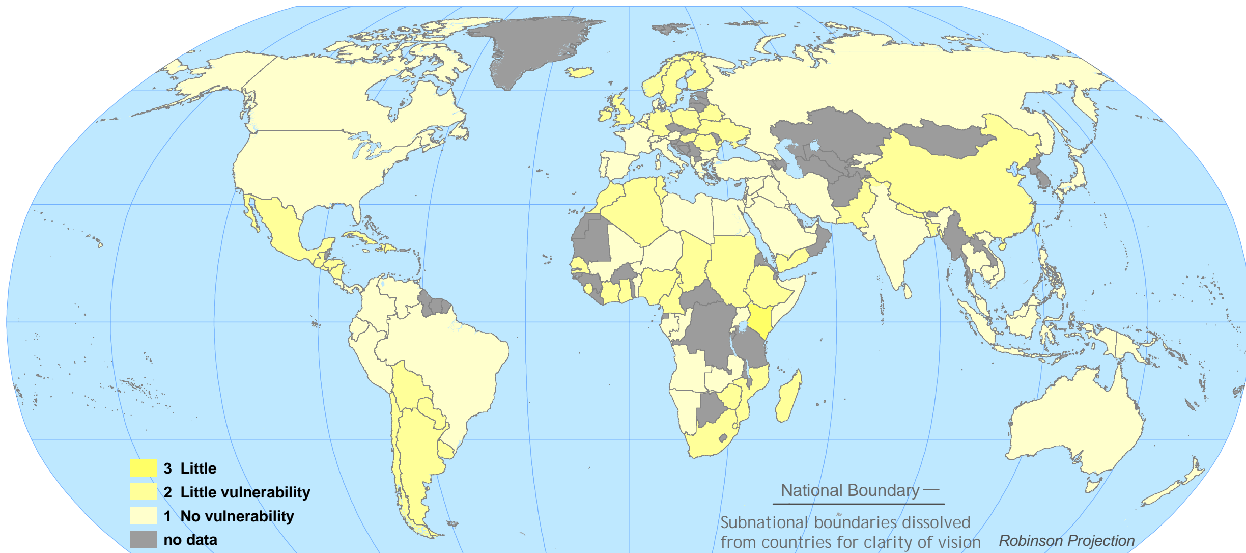
Scenario A2 in Year 2050 with Climate Sensitivity Equal to 1.5 Degrees C DJF Mean Temperature with Aggregate Impacts Calibration and Enhanced Adaptive Capacity
