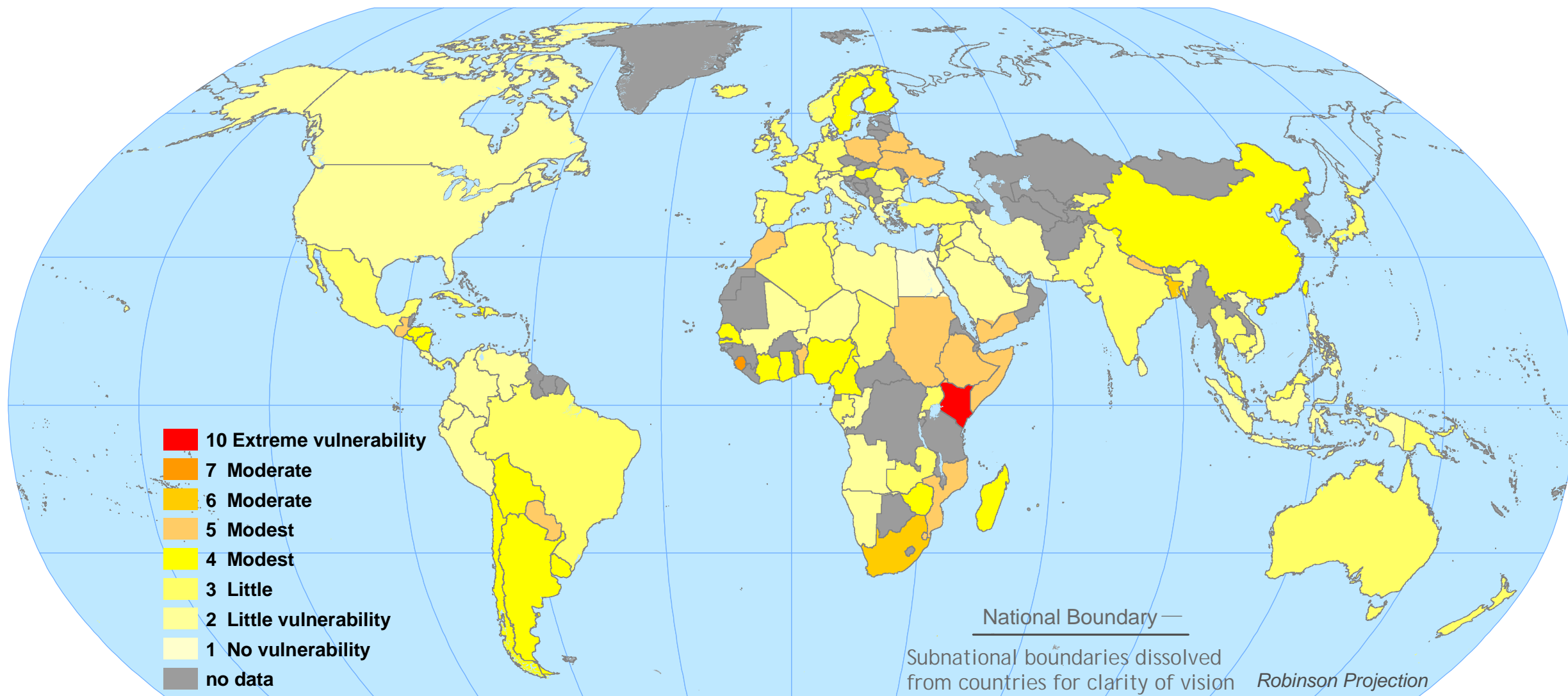
Scenario A2-550 in Year 2050 with Climate Sensitivity Equal to 5.5 Degrees C DJF Mean Temperature with Aggregate Impacts Calibration
