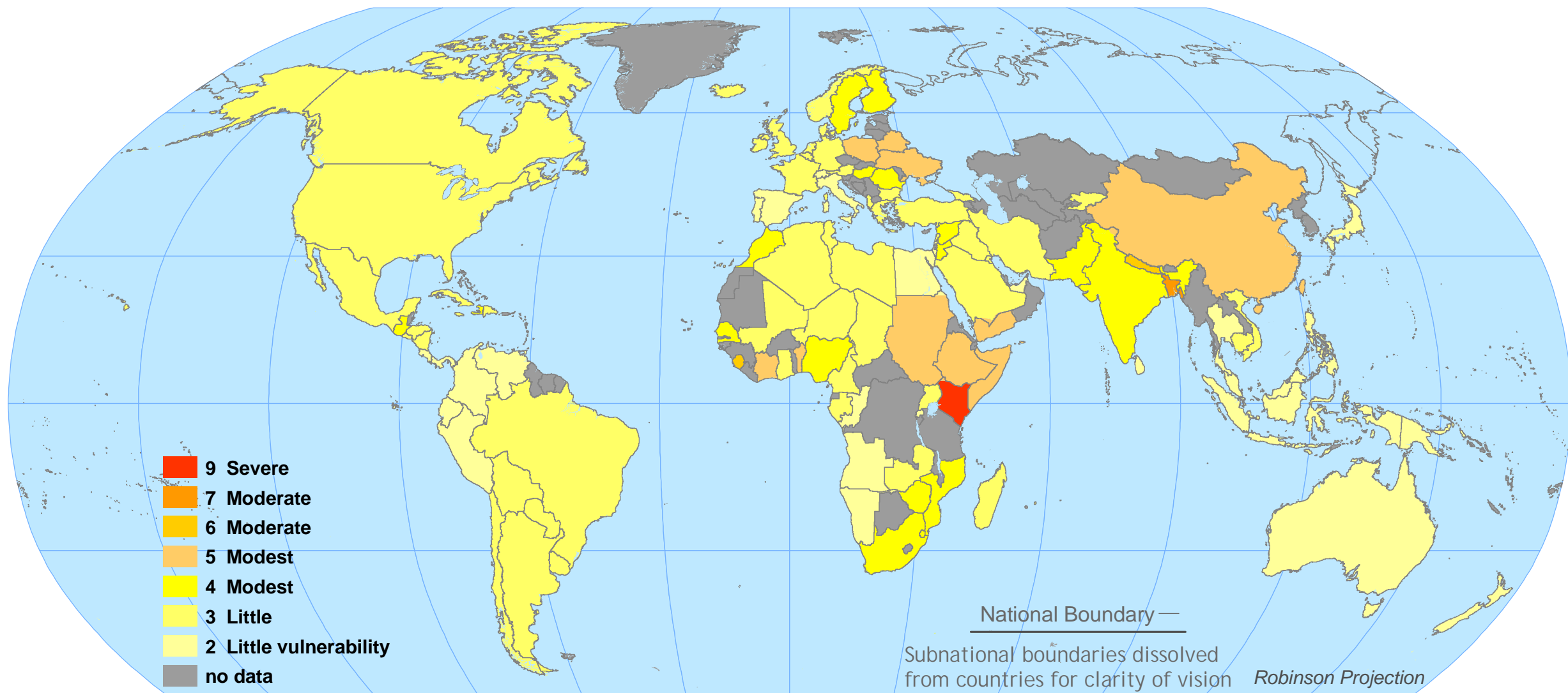
Scenario A2-550 in Year 2100 with Climate Sensitivity Equal to 1.5 Degrees C DJF Mean Temperature with Aggregate Impacts Calibration
