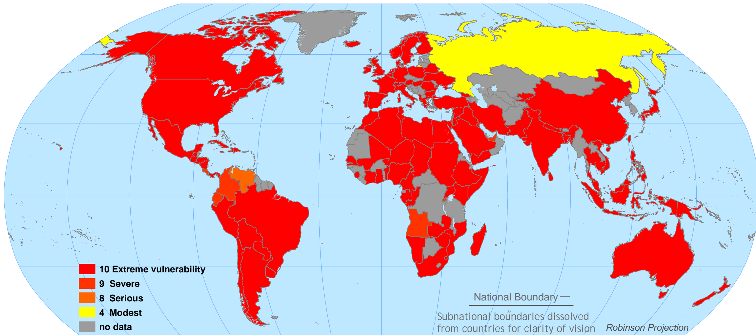
Scenario A2 in Year 2100 with Climate Sensitivity Equal to 5.5 Degrees C DJF Mean Temperature with Extreme Events Calibration and Enhanced Adaptive Capacity
