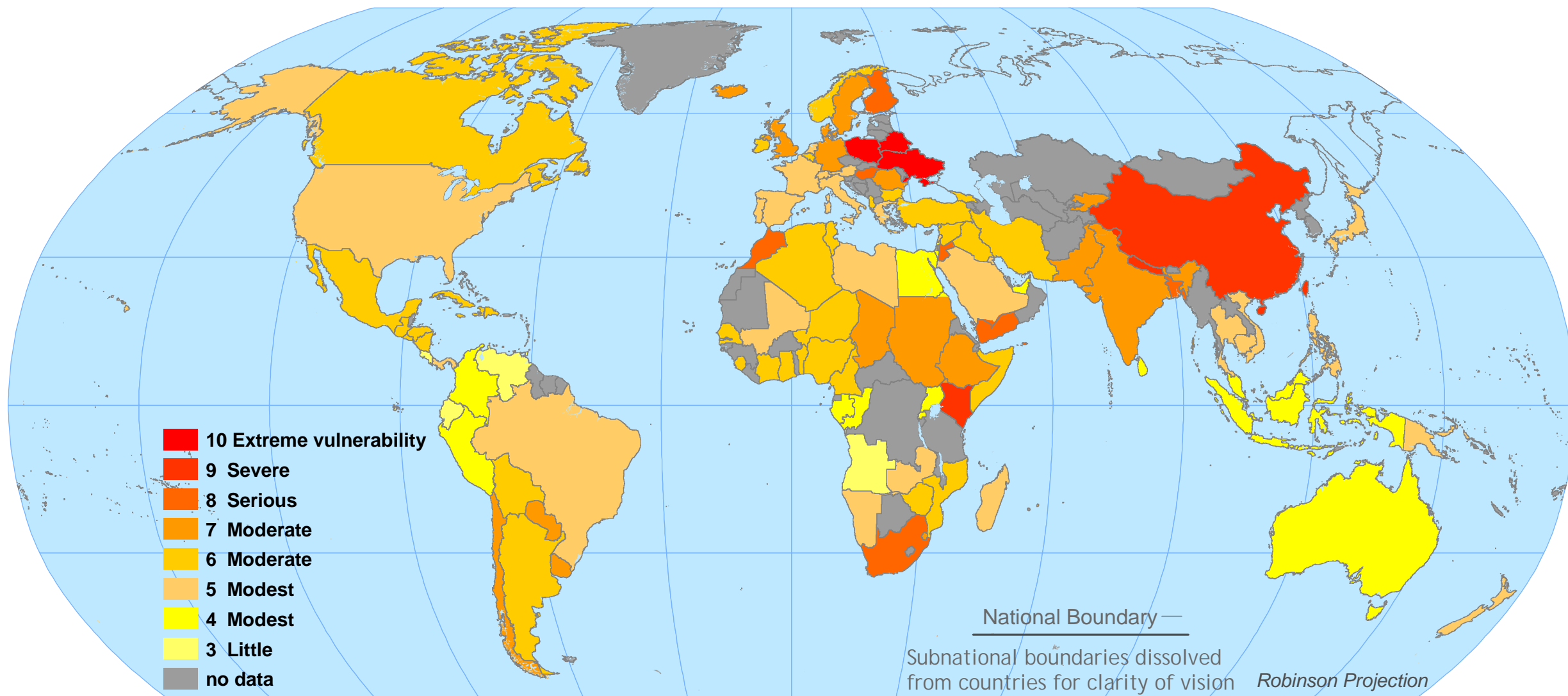
Scenario A2-550 in Year 2100 with Climate Sensitivity Equal to 5.5 Degrees C DJF Mean Temperature with Aggregate Impacts Calibration and Enhanced Adaptive Capacity
