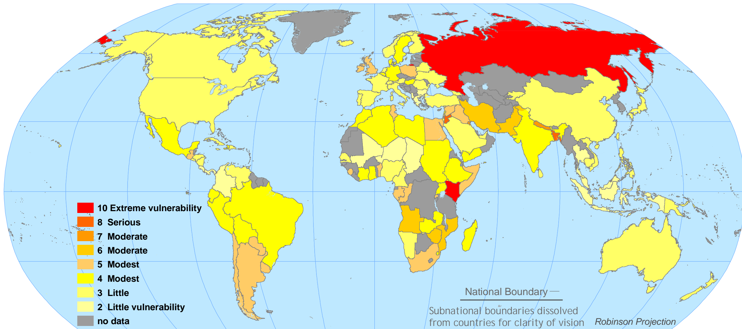
Scenario A2 Year 2050 with Climate Sensitivity Equal to 5.5 Degrees C JJA Mean Temperature with Aggregate Impacts Calibration
