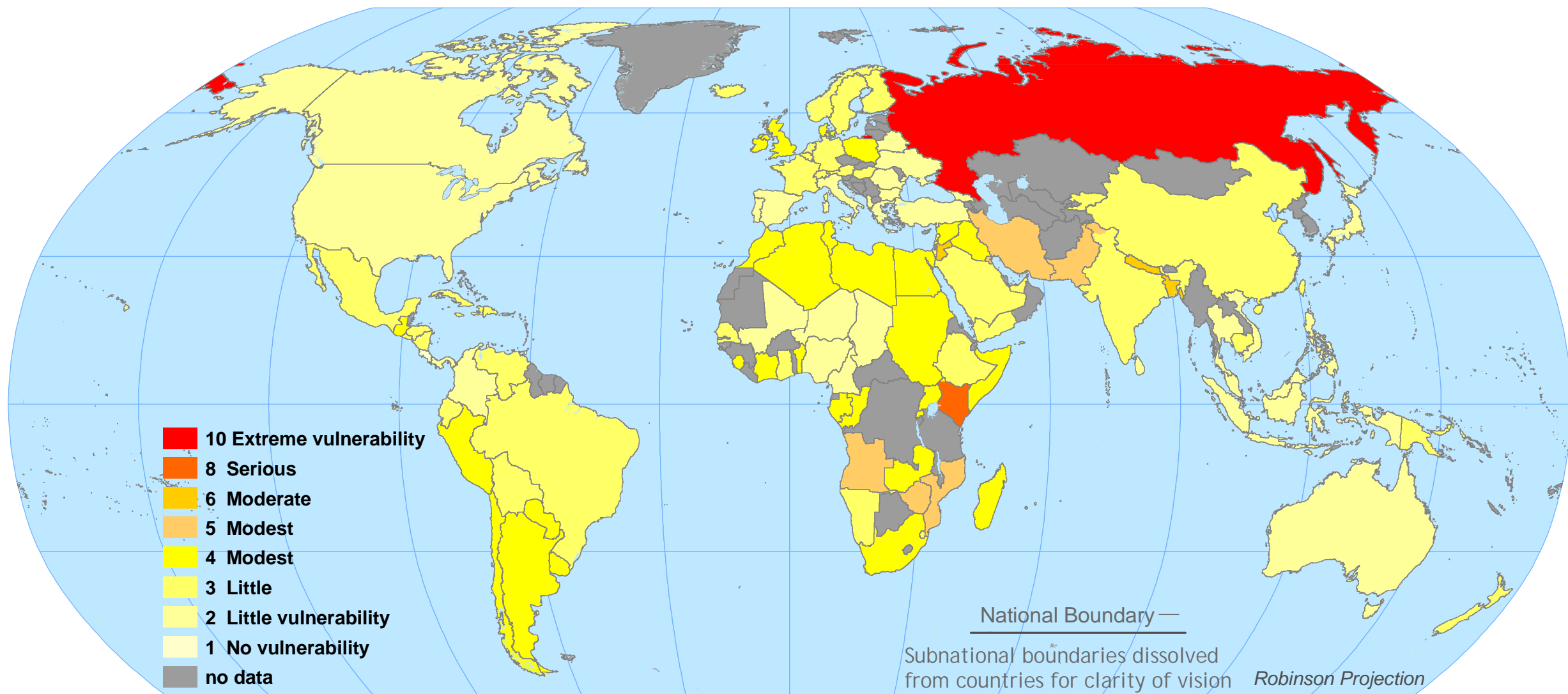
Scenario A2-550 in Year 2050 with Climate Sensitivity Equal to 5.5 Degrees C JJA Mean Temperature with Aggregate Impacts Calibration
