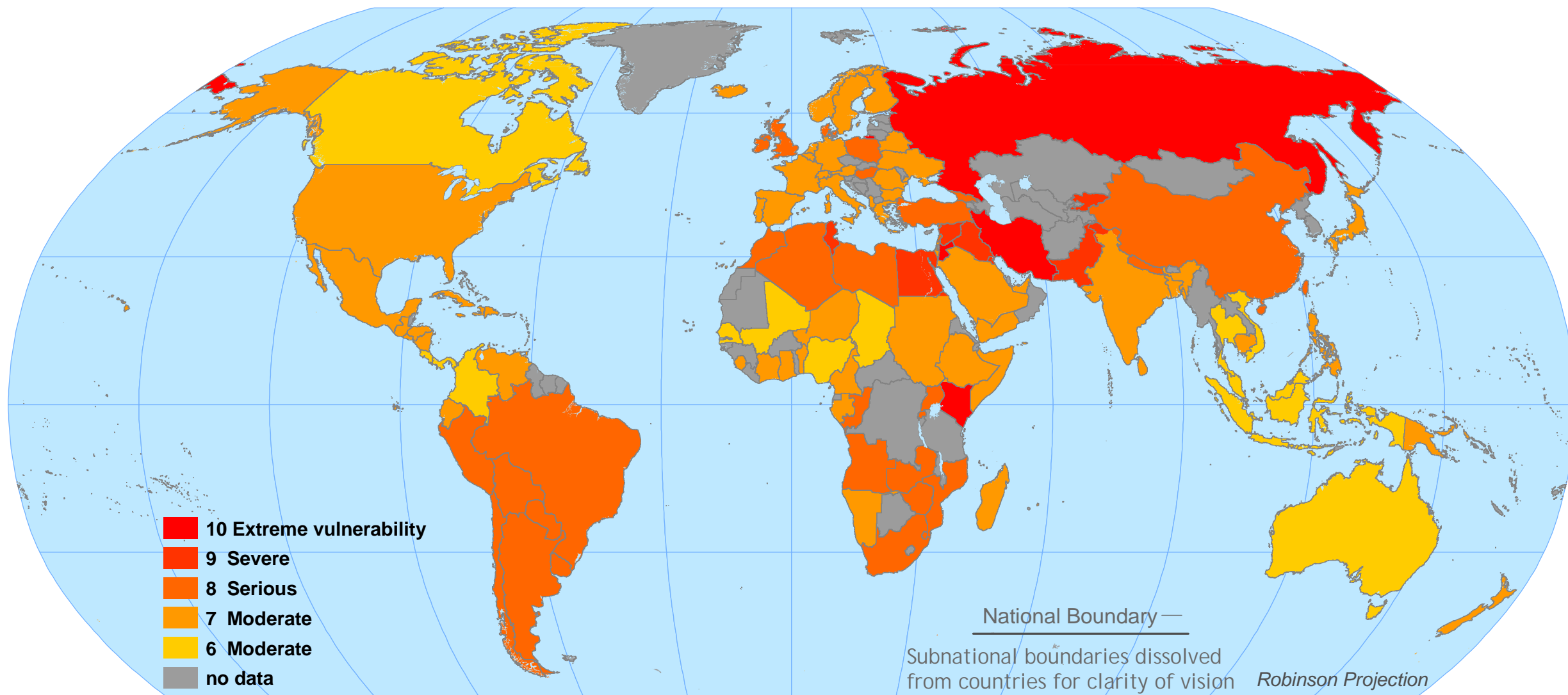
Scenario B2 in Year 2050 with Climate Sensitivity Equal to 5.5 Degrees C JJA Mean Temperature with Extreme Events Calibration and Enhanced Adaptive Capacity
