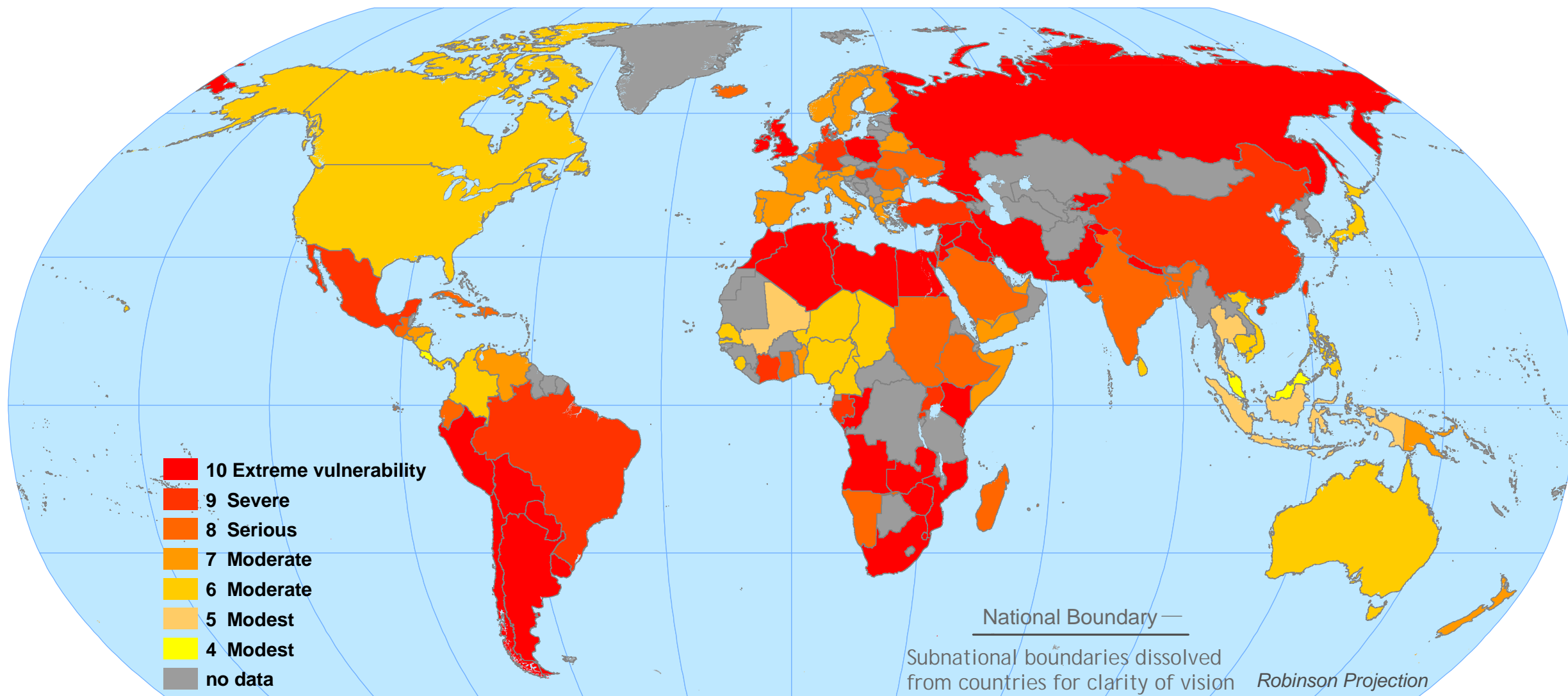
Scenario A2 in Year 2100 with Climate Sensitivity Equal to 5.5 Degrees C JJA Mean Temperature with Aggregate Impacts Calibration and Enhanced Adaptive Capacity
