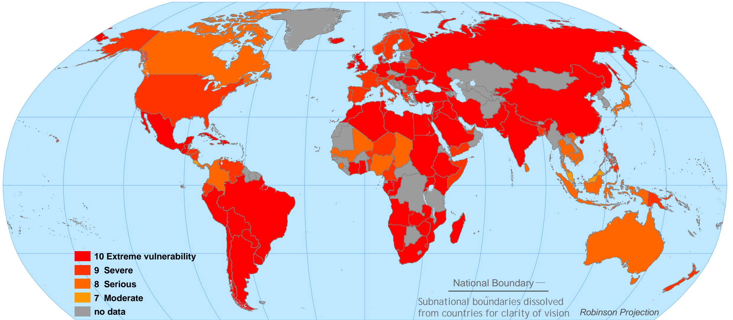
Scenario B2 in Year 2100 with Climate Sensitivity Equal to 5.5 Degrees C JJA Mean Temperature with Extreme Events Calibration and Enhanced Adaptive Capacity
