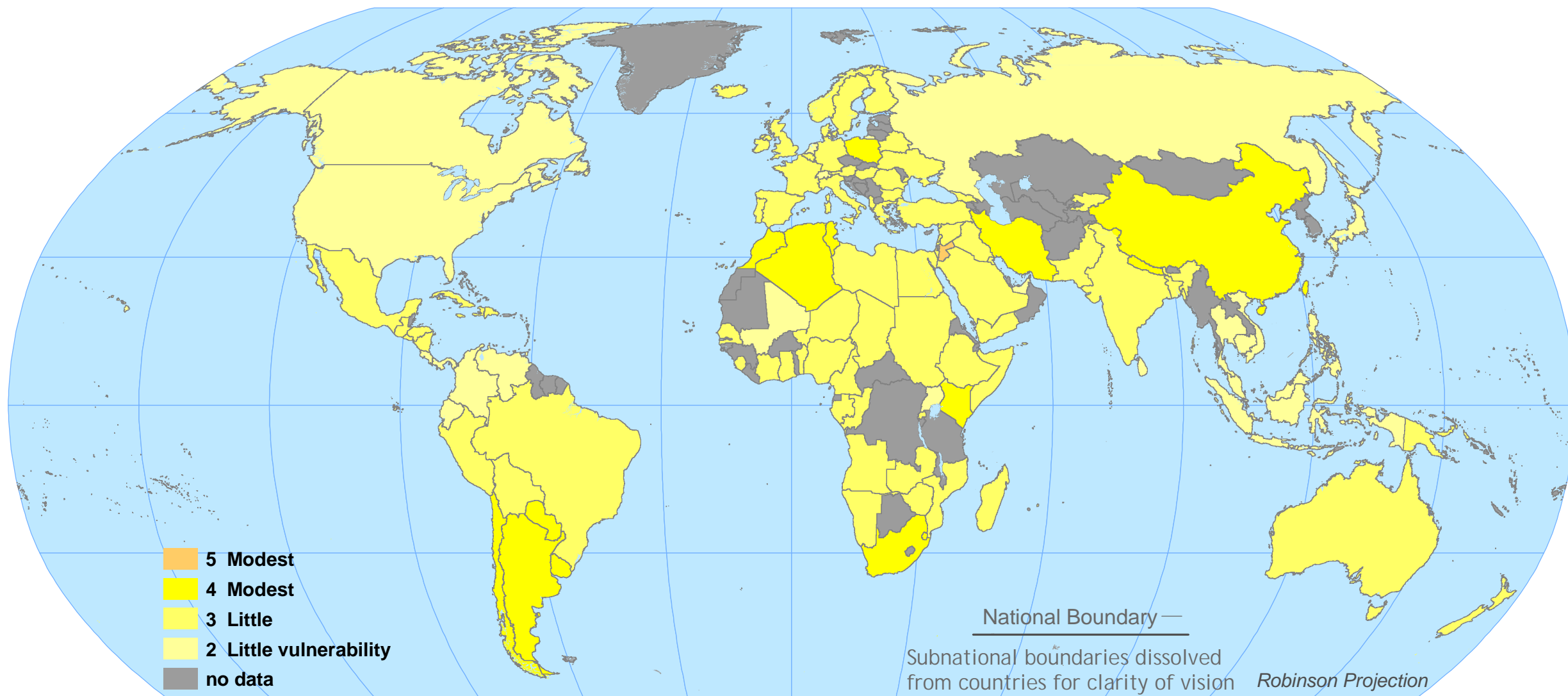
Scenario A2 Year 2050 with Climate Sensitivity Equal to 5.5 Degrees C Annual Mean Temperature with Aggregate Impacts Calibration and Enhanced Adaptive Capacity
