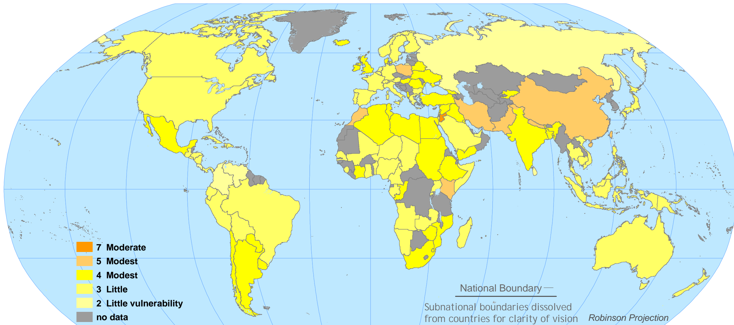
Scenario B2 in Year 2050 with Climate Sensitivity Equal to 5.5 Degrees C Annual Mean Temperature with Aggregate Impacts Calibration and Enhanced Adaptive Capacity
