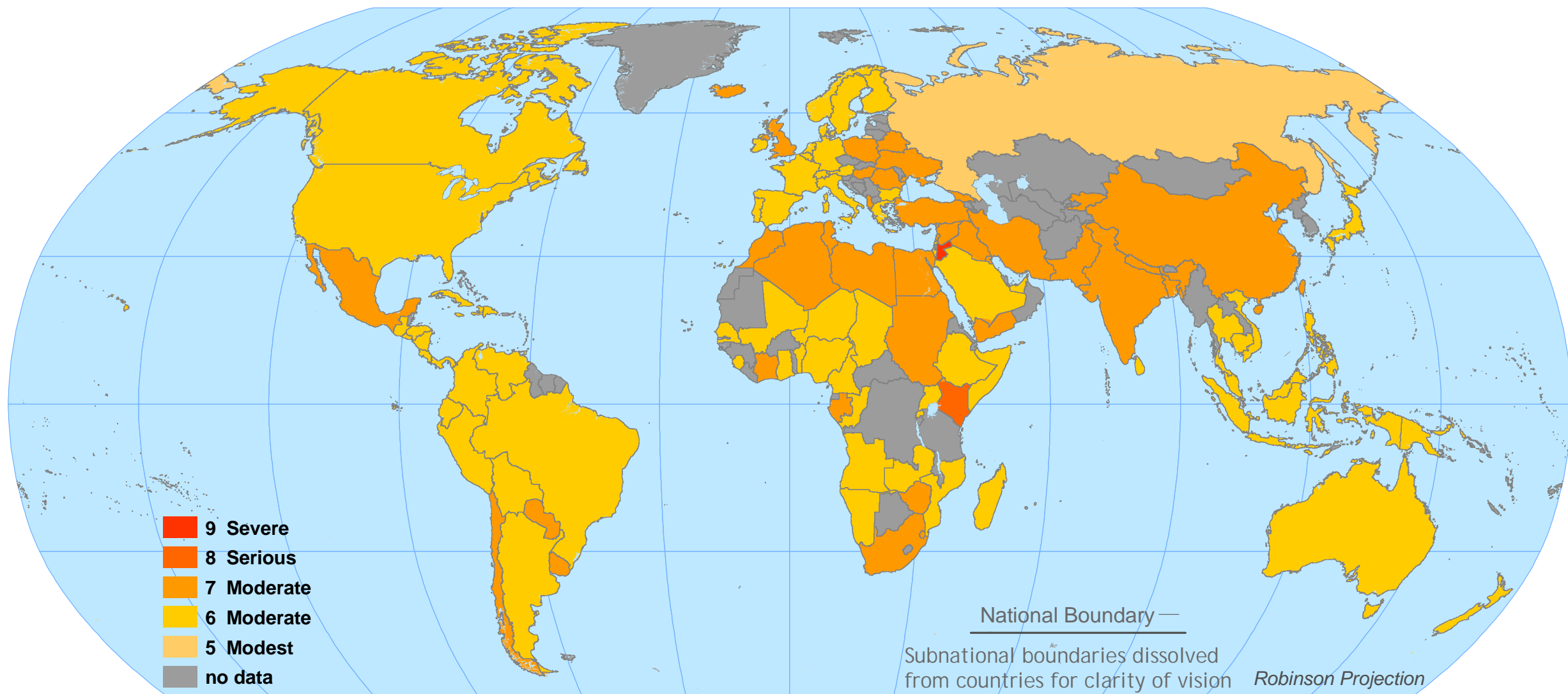
Scenario A2-550 in Year 2100 with Climate Sensitivity Equal to 1.5 Degrees C Annual Mean Temperature with Extreme Events Calibration and Enhanced Adaptive Capacity
