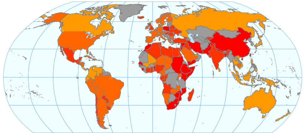
Scenario B2 in Year 2050 with Climate Sensitivity Equal to 5.5 Degrees C Annual Mean Temperature with Extreme Events Calibration
