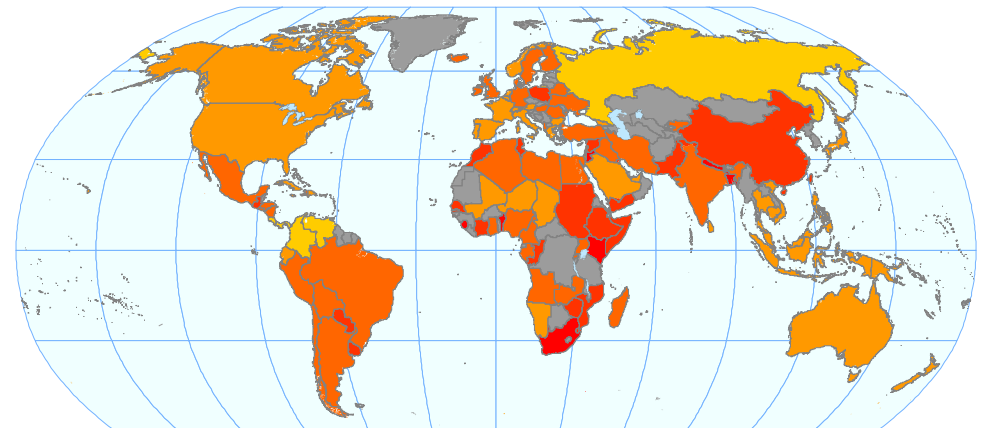
Scenario A2 in Year 2050 with Climate Sensitivity Equal to 5.5 Degrees C Annual Mean Temperature with Extreme Events Calibration
